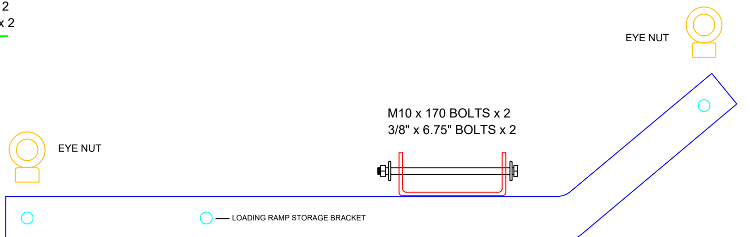
FRONT TIE DOWN BAR CURVED END FACES AWAY FROM VEHICLE
