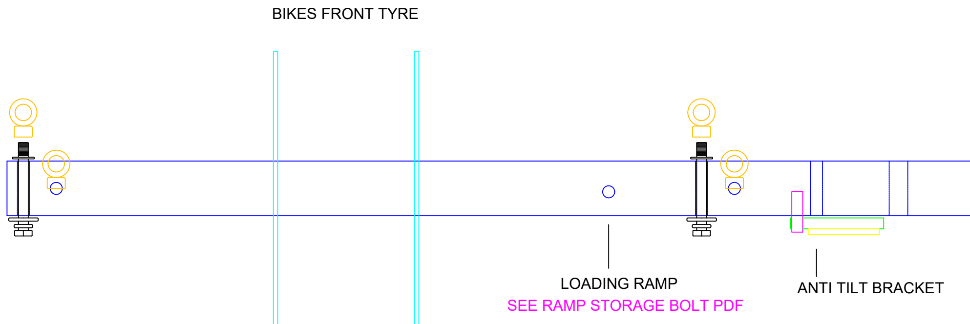
MAIN BAR TOP VIEW
